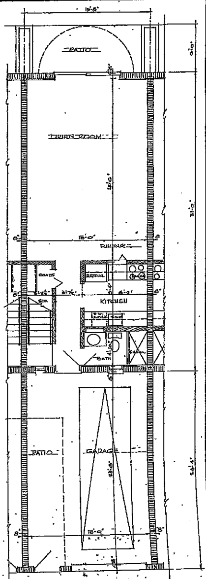
TYPICAL FIRST FLOOR PLAN Scale 1/8" = 1'-0"
