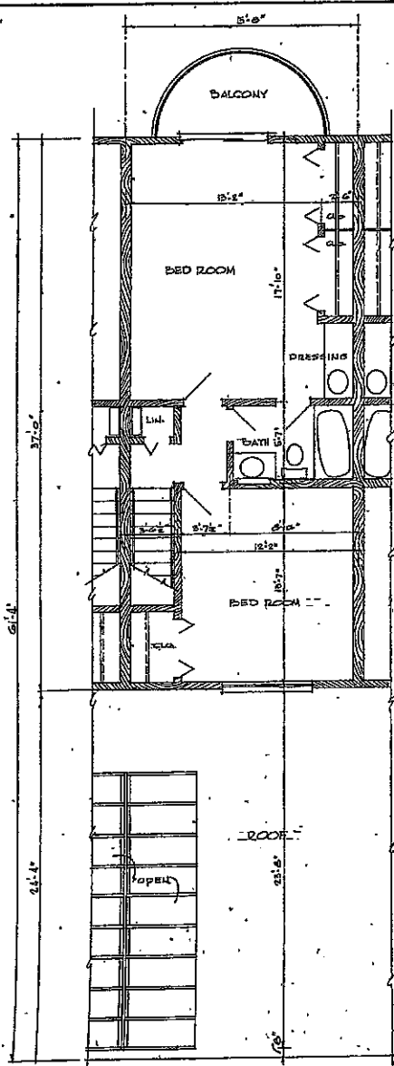
TYPICAL SECOND FLOOR PLAN Scale 1/8" = 1'-0"
